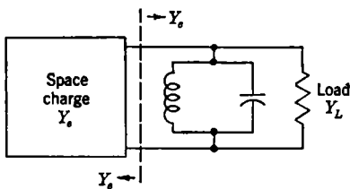
FIG. 8-26.—Equivalent circuit of a magnetron.
